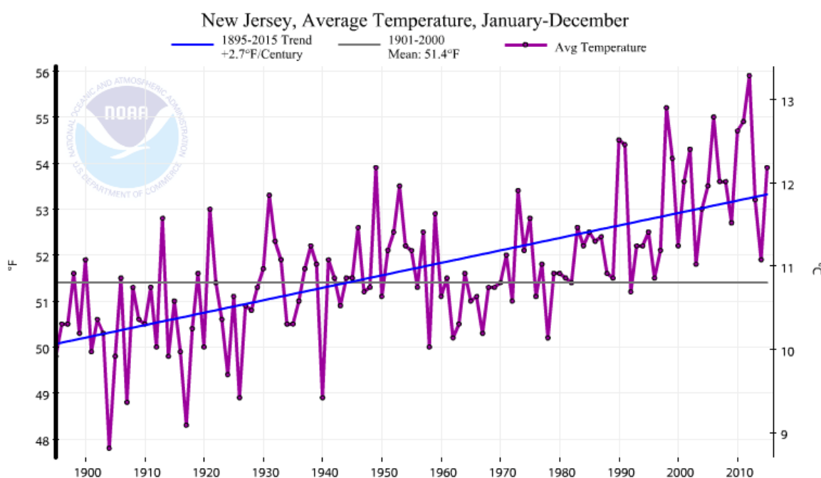
Figure 4: New Jersey Statewide Average Annual Temperature, 1895-2015
