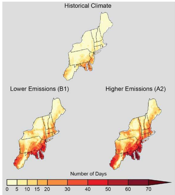
Figure 11: Projected Increases in the Number of Days over 90°F
