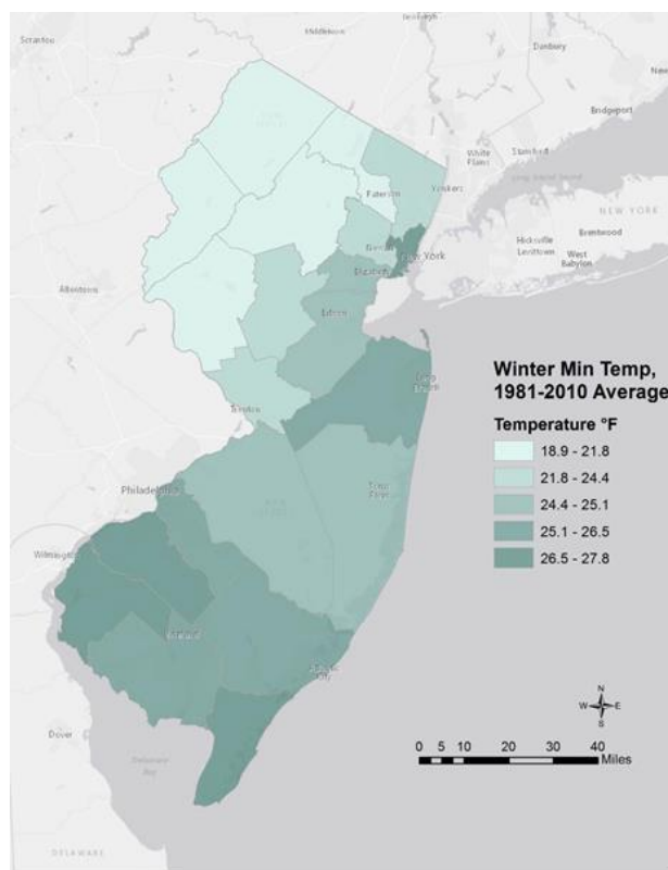
Figure 6: New Jersey Winter Minimum Temperature, 1981-2010 in °F
