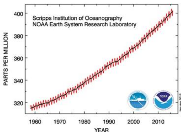
Figure 3: Atmospheric CO 2 Concentrations Measured at Mauna Loa Observatory
