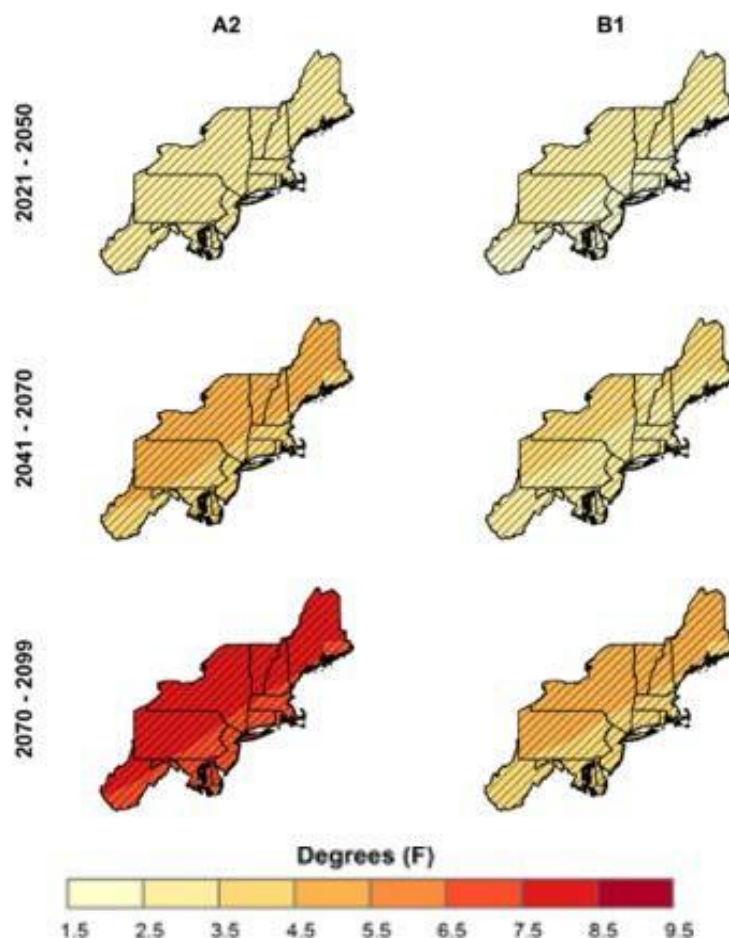
Figure 10: Multi-Model Mean Annual Temperature Projections in °F, Anomalies Relative to 1971-1999 Average
