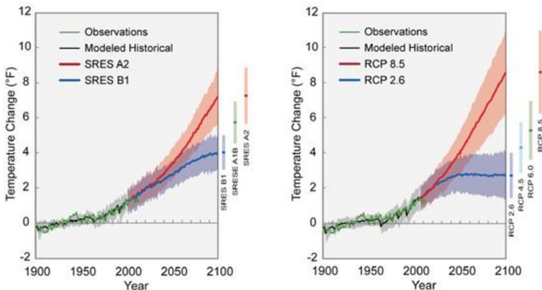
Figure 9: Comparison of Low (B1 and RCP 2.6) and High (A2 and RCP 8.5) Range Emissions Scenarios for RCP and SRES
