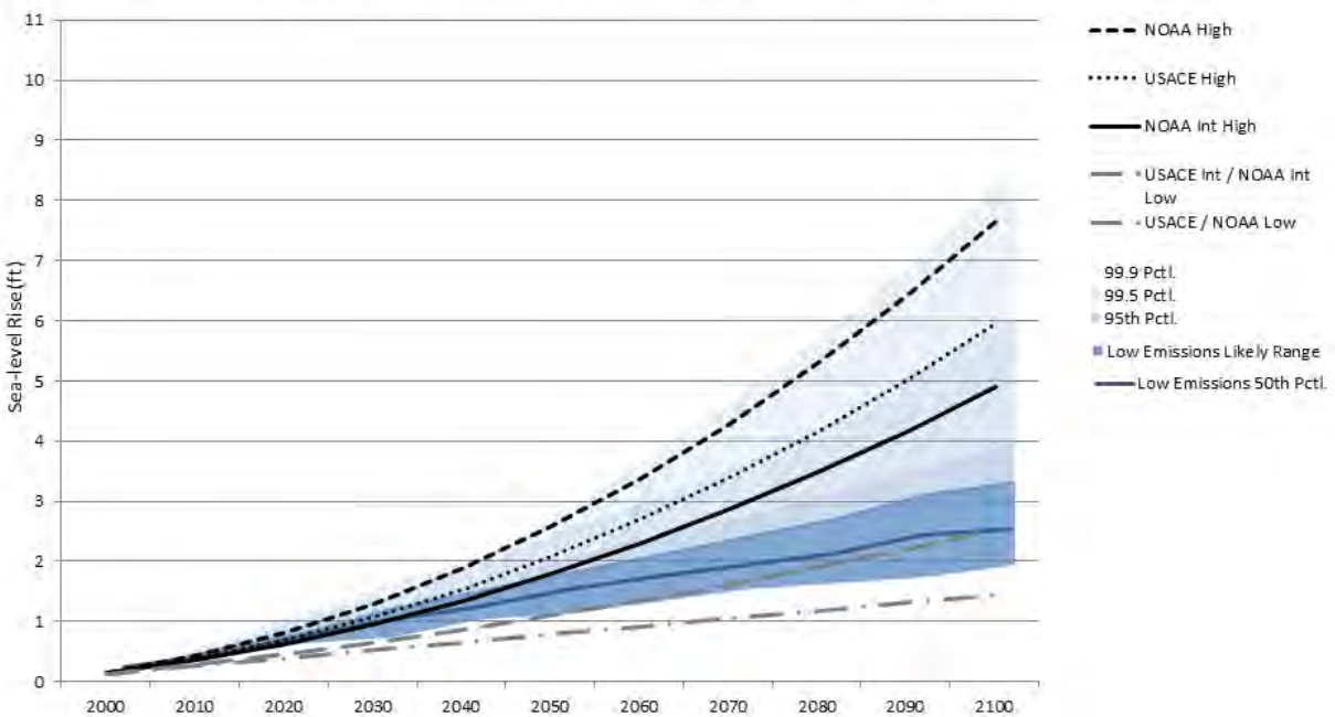
Figures 1a and 1b: SLR Projections for New Jersey (Atlantic City) Compared to Federal Projections: Projections for high-emissions (red) and low-emissions scenarios (blue), based on (Kopp et al., 2014). Solid Lines = 50 th percentile; Shaded Area = likely ranges (17 th – 83 rd percentile); 83 rd – 95 th percentile, 95 th – 99.5 th percentile, and 99.5 th – 99.9 th percentile. All sea levels are with respect to a 1991-2009 baseline. Note that these results represent a single way of estimating the probability of different levels of SLR; alternative methods may yield higher or lower estimates of the probability of high-end outcomes. Federal projections are based on data from the Sea-Level Change Curve Calculator (2015.46) available at http://www.corpsclimate.us/ccaceslcurves.cfm . Federal estimates are expressed
